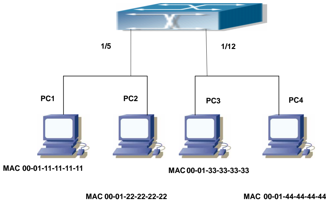
Fig 6-1 MAC Table dynamic learning
