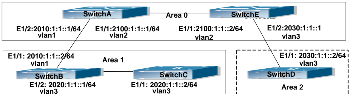
Fig 17-9 Network topology of OSPF autonomous system.
