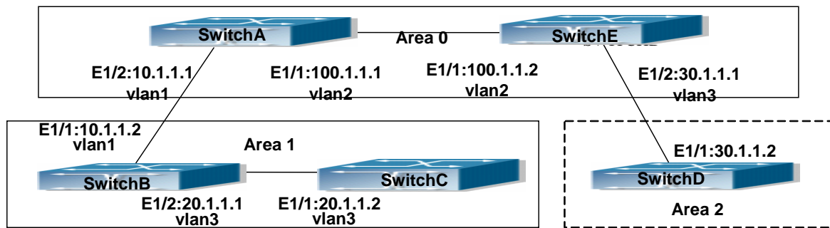
Fig 17-6 Network topology of OSPF autonomous system.
