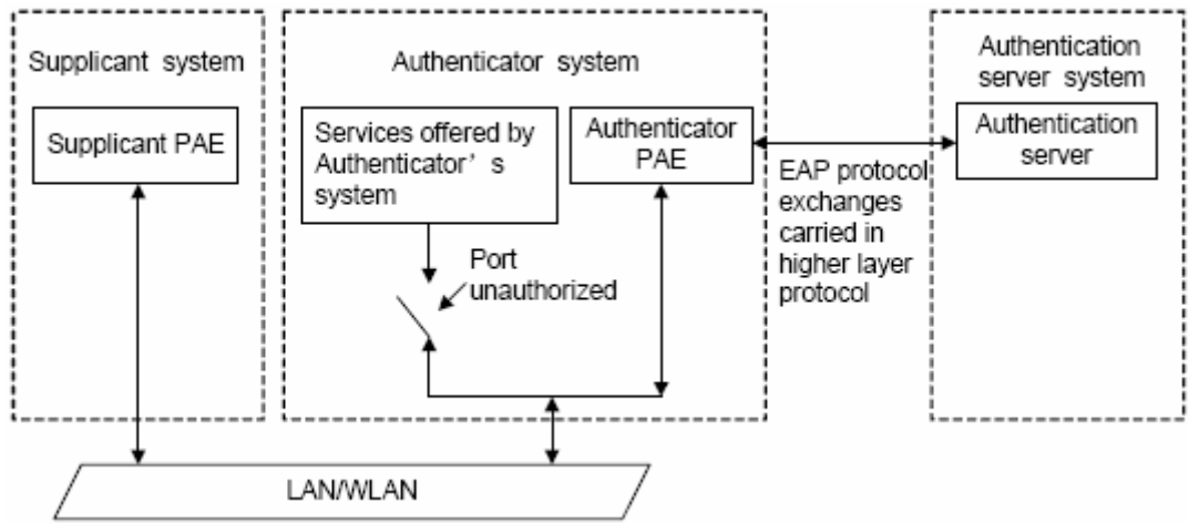
Fig 23-1 The Authentication Structure of 802.1x
