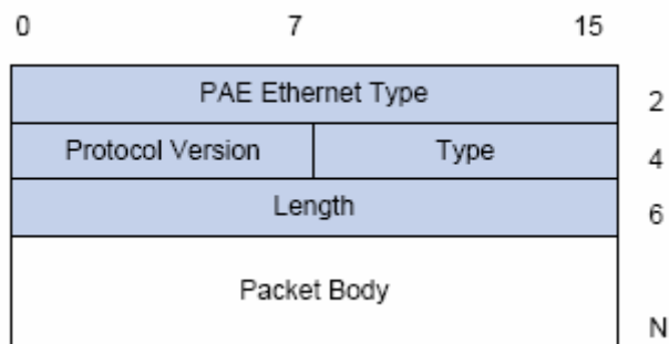
Fig 23-3 the Format of EAPOL Data Packet
