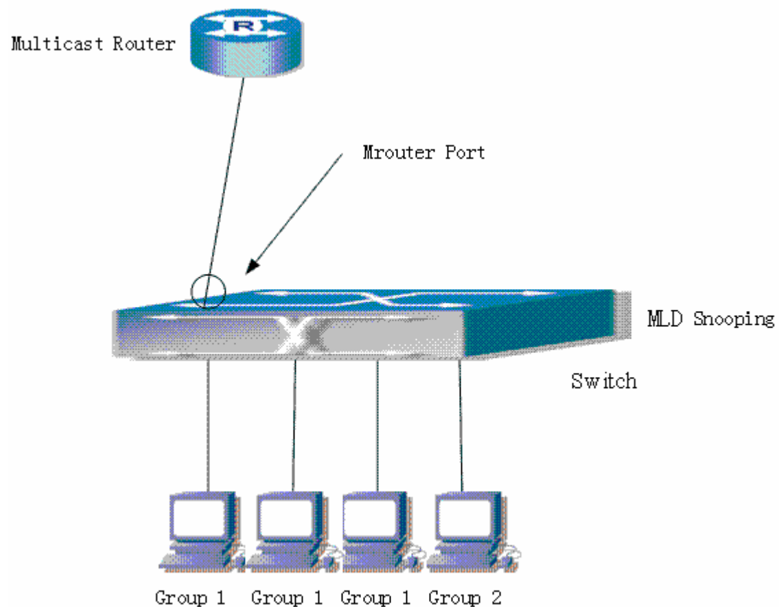
Fig 21-4 Open the switch MLD Snooping Function figure
