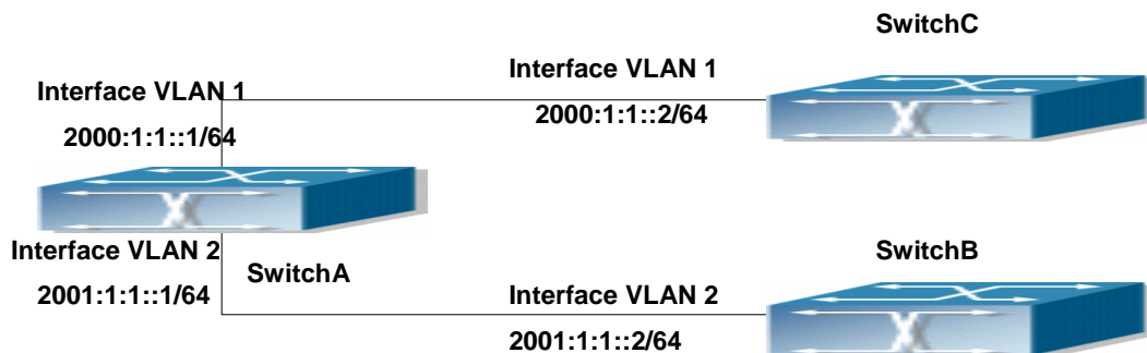
Fig 17-5 RIPng Example
