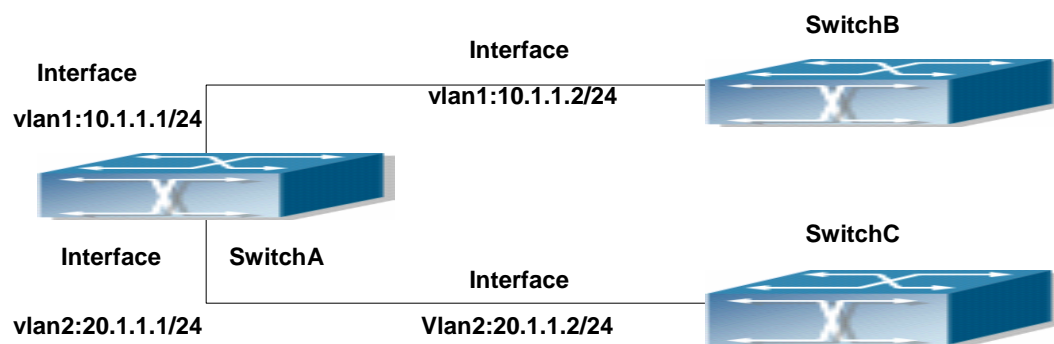
Fig 17-3 RIP example
