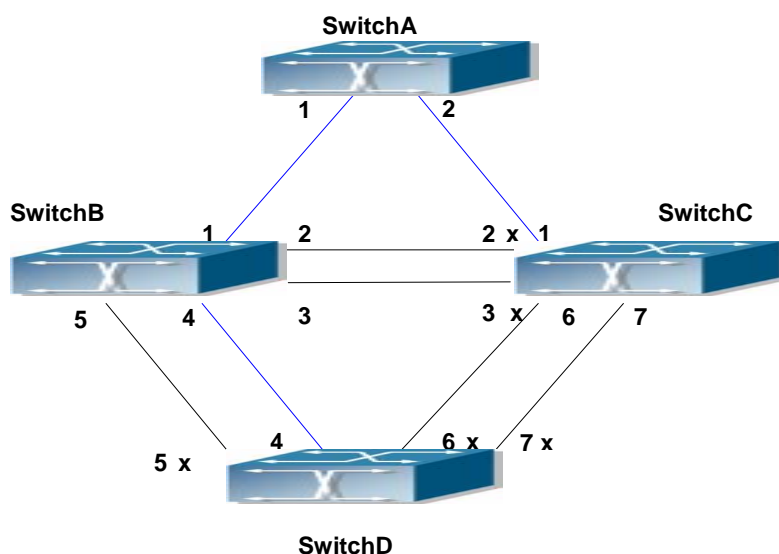
Fig 7-2 Typical MSTP Application Scenario
