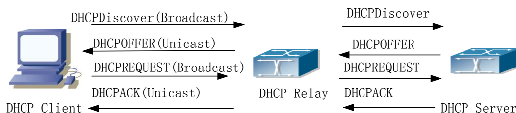
Fig 10-2 DHCP relay
