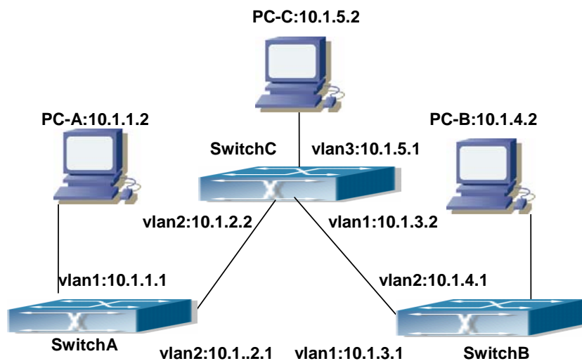
Fig 17-2 Static Route Configurations
