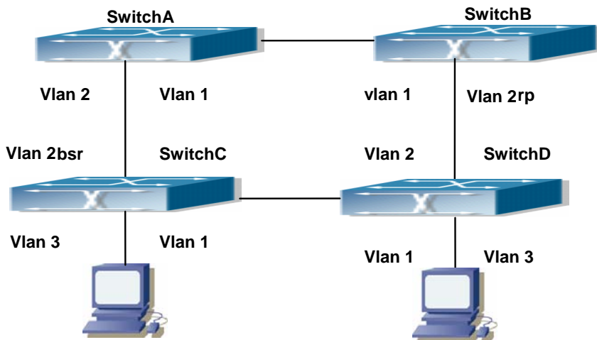
Fig 21-2 PIM-SM Typical Environment
