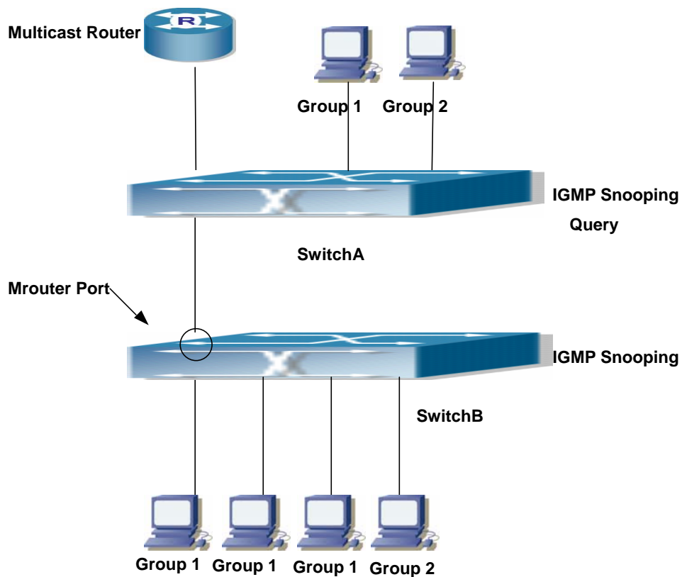
Fig 18-2 The switches as IGMP Queriers
